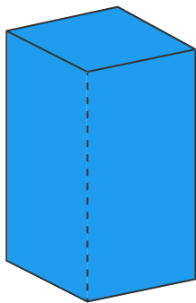
cuboid
