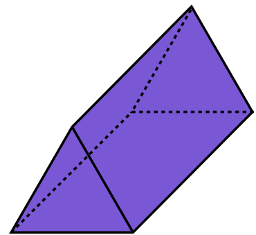
triangular prism
