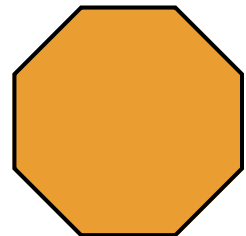
octagon
