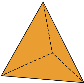
tetrahedron/ triangular based pyramid
