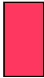
rectangle
