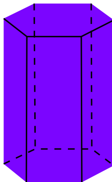
hexagonal prism
