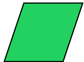
parallelogram
